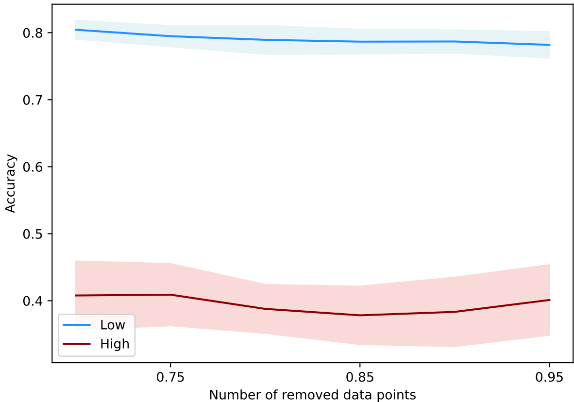
DataAttrOpt(5000, 0.03, 15, best, +b, alpha=best) - imdb-embeddings
